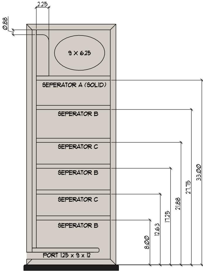
SIDE VIEW
